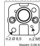
Alluminium adapter flange Code: E60513025
